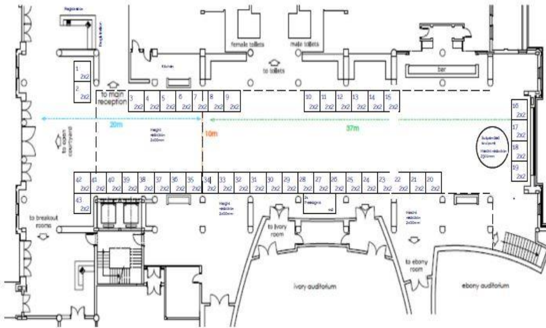
The Forum Foyer 1:200
